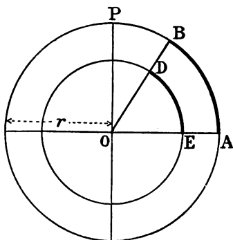
FIG. 21.—Measurement of an angle in radians.
