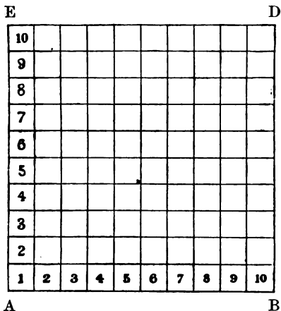
FIG. 4.—Representing a square metre divided into 10 decimetres. Scale \frac{1}{10} .
