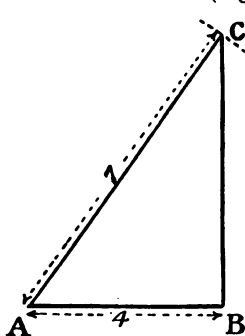
FIG. 65.—Given the cosine of an angle to construct the angle.
