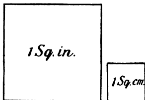
FIG. 3.—Square inch and square centimetre.
