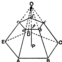
FIG. 160.—Frustum of a pyramid.
