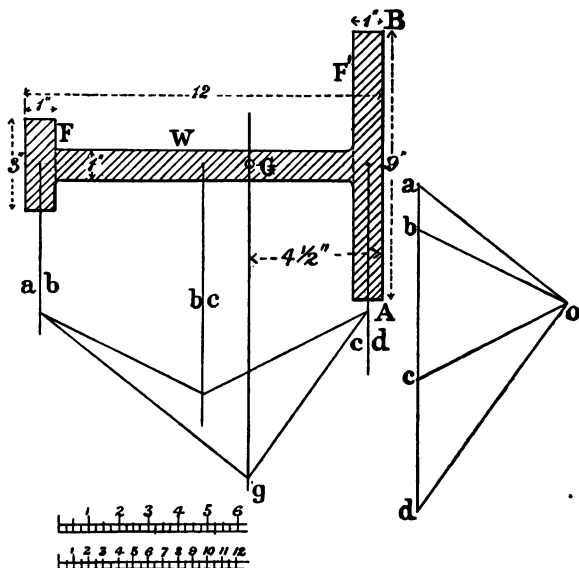
FIG. 177.—Centre of area.
