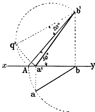
FIG. 92.—To obtain the projections of a line given its true length and inclinations.
