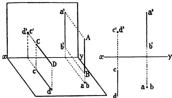
FIG. 81.—Projections of a line, perpendicular to one plane, and parallel to the other.
