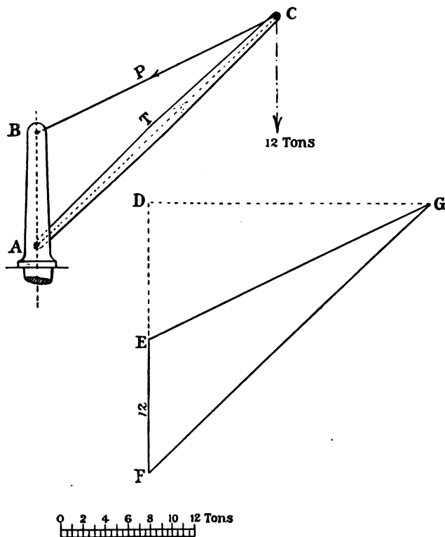
FIG. 169.—Ordinary crane.
