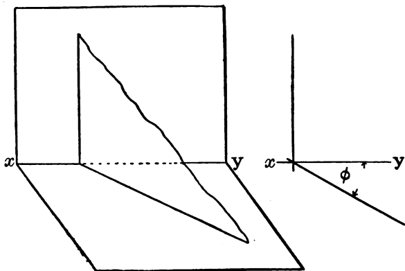
FIG. 96.—Vertical Plane.
