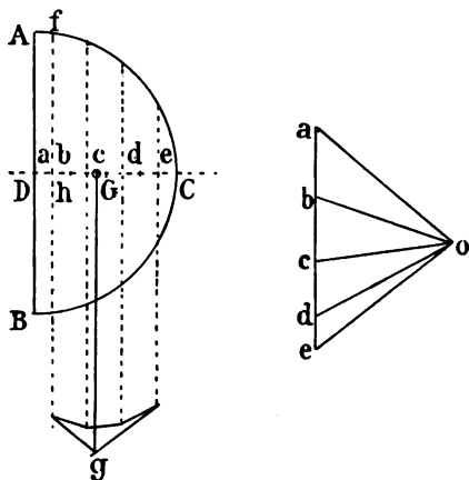
FIG. 178.—Centre of area of a semicircle.
