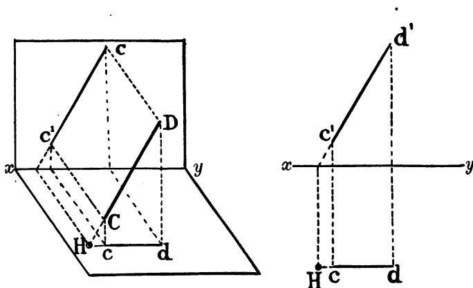
FIG. 83. — Projections of a line, parallel to V.P., inclined to the H.P.
