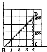
FIG. 199.—Work done in slowly compressing a spiral spring.
