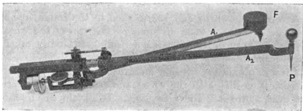
FIG. 138.—The Planimeter.
