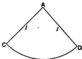
FIG. 163.—Development of a cone.
