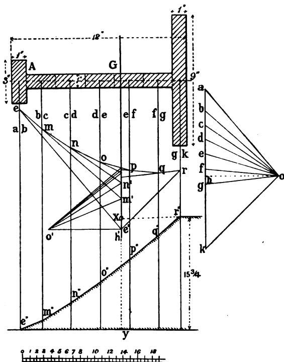
FIG. 185.—Moment of inertia obtained graphically.
