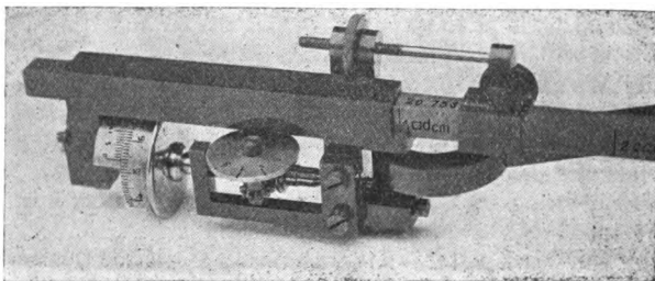
FIG. 139.—Planimeter showing the vernier arrangement.
