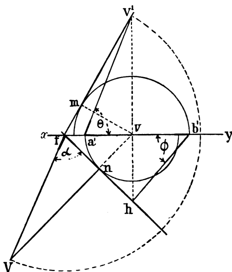
FIG. 97.—Inclinations: Oblique Plane.
