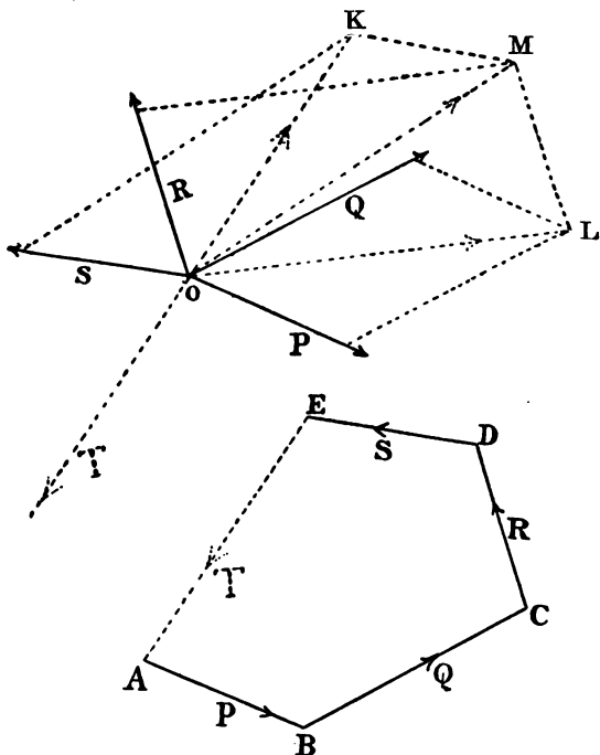
FIG. 171.—Sum of vectors acting at a point.
