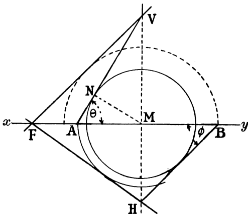
FIG. 98.—Given inclination of a plane to obtain its traces.
