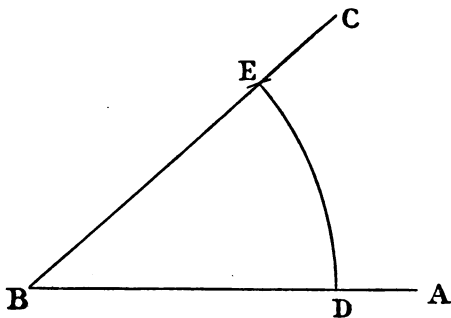
FIG. 20.—To measure the magnitude of an angle.
