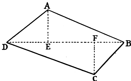
FIG. 119.—Area of a quadrilateral.
