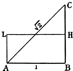
FIG. 115.—Area of an isosceles triangle.
