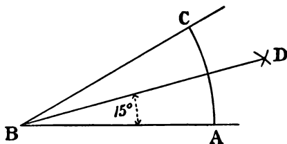
FIG. 16.—To set out an angle of 15^\circ .
