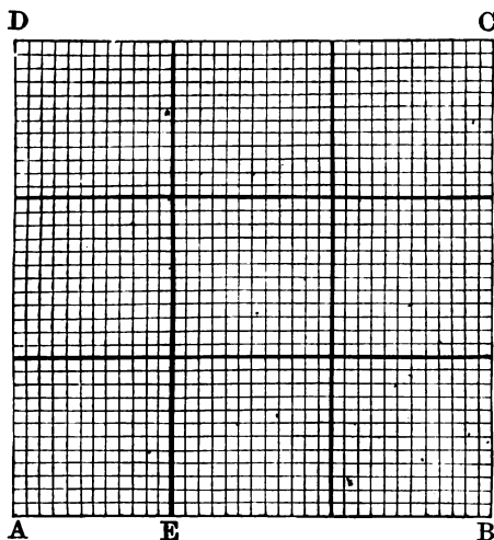
FIG. 2.—1 square yard equals 9 square feet, or 9 \times 144 square inches.
