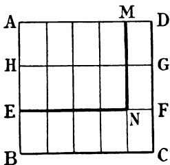
FIG. 33.—To show that \frac{4}{5} of \frac{2}{3} = \frac{8}{15} .
