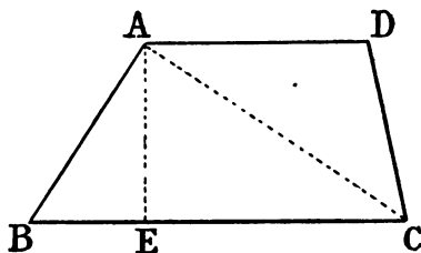
FIG. 121.—Area of a trapezium.
