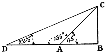
FIG. 62.—Angle of 22\frac{1}{2}^\circ and 67\frac{1}{2}^\circ .
