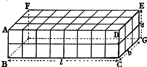
FIG. 144.—Volume of a right prism or parallelepiped.
