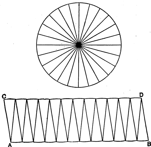
FIG. 124.—Area of a circle.
