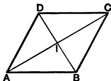
FIG. 118.—Area of a rhombus.
