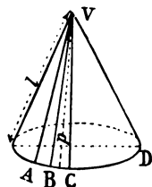
FIG. 162.—Lateral surface of a cone.
