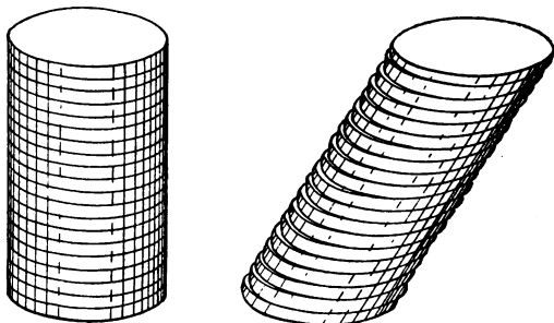
FIG. 152.—Model to illustrate a right and an oblique cylinder.
