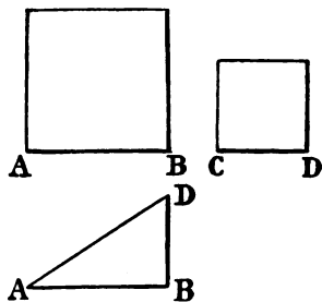
FIG. 110.—Addition and subtraction of areas.
