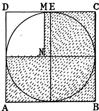
FIG. 125.—Area of a circle experimentally.
