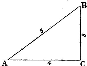
FIG. 22.—The three angles of a triangle are together equal to 180^\circ .
