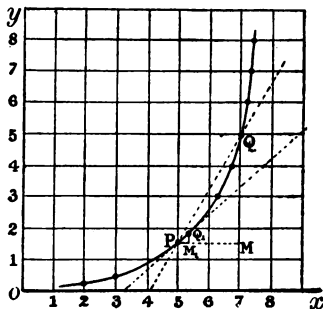
FIG. 197.—Slope of a curve.
