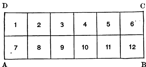
FIG. 111.—Area of a rectangle.
