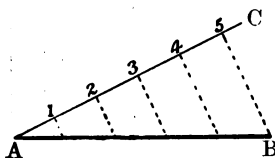
FIG. 35.—Division of a line.
