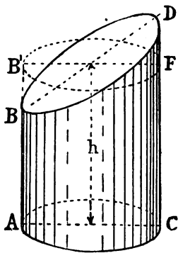
FIG. 153.—Frustum of a cylinder.
