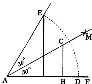
FIG. 55.—Angle of 30^\circ .
