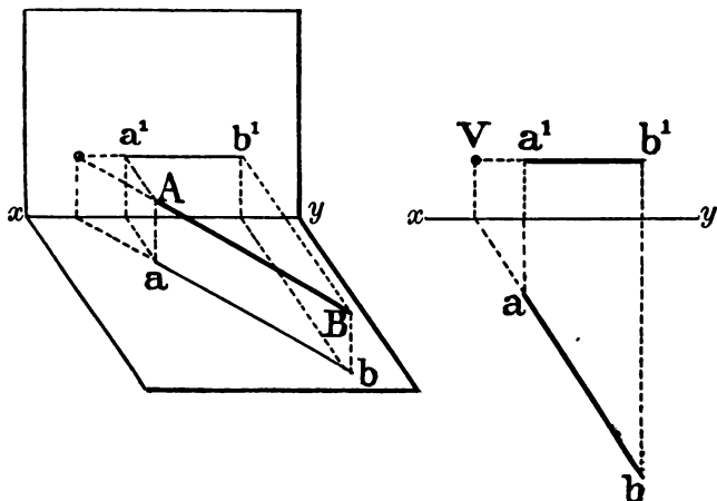
FIG. 82.—Projections of a line parallel to H.P. inclined to V.P.
