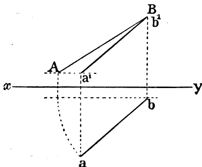
FIG. 86.—Given the projections of a line to determine its true length and inclination to the H.P.
