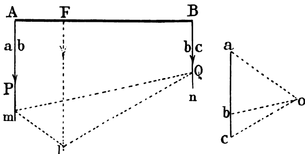
FIG. 174.—Parallel forces.
