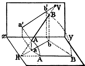
FIG. 84.—Line inclined to both planes of projection.
