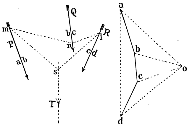
FIG. 173.—Forces not acting at a point.
