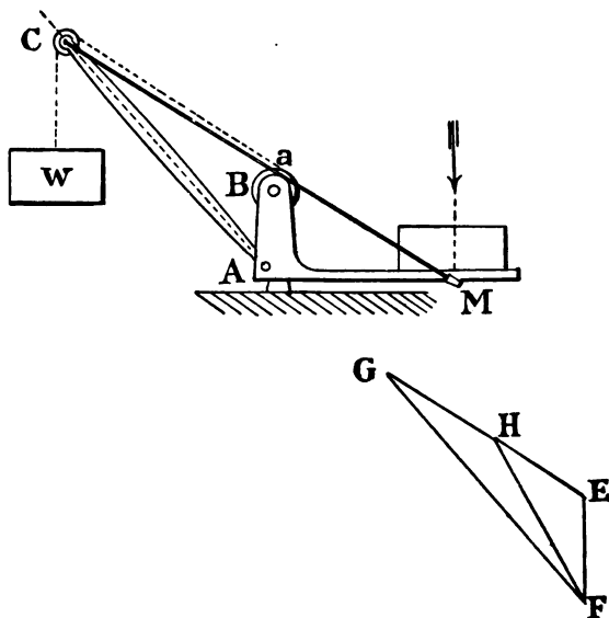
FIG. 170.—Wharf crane.
