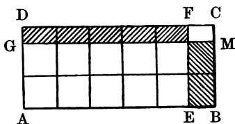
FIG. 112.—Area of a rectangle.
