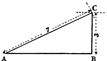
FIG. 64.—Given the sine of an angle to construct the angle.
