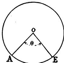
FIG. 128.—Area of sector of a circle.
