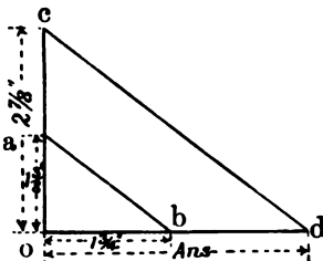
FIG. 41.—Simplification of a fraction.
