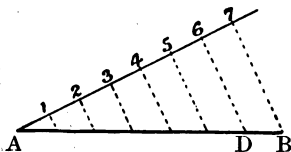
FIG. 36.—To find the unit of length, when a line AB represents 7 units.
