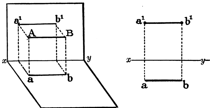
FIG. 80.—Projections of a line parallel to both planes of projection.
