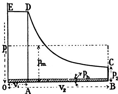
FIG. 201.—Area enclosed by hyperbolic curve.
