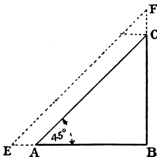
FIG. 57.—Angle of 45^\circ .
