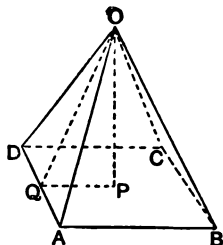
FIG. 159.—Surface of a pyramid.
