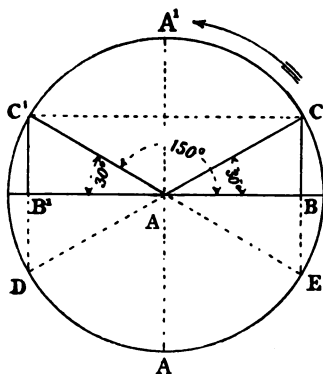
FIG. 60.—Angles greater than 90^\circ .
