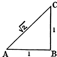
FIG. 59.—Isosceles right-angled triangle.
