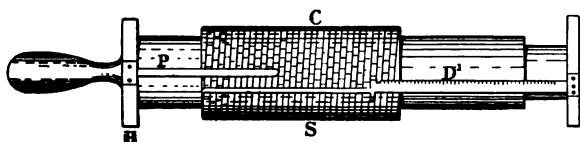
FIG. 74.—Fuller's slide-rule.
