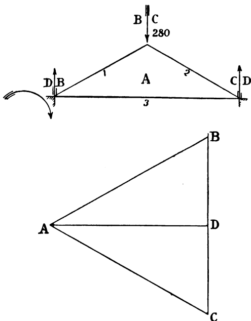
FIG. 181.—Couple-close roof truss.
