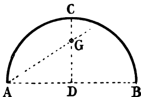
FIG. 176. —Centre of gravity of a curved line.
