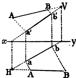
FIG. 85.—Projections of a line inclined to both planes of projection.
