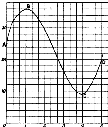
FIG. 196.—Curve showing maximum and minimum values.
