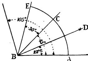
FIG. 17.—To set out an angle of 22\frac{1}{2}^\circ .
