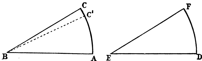
FIG. 14.—Comparison of the magnitudes of two angles.
