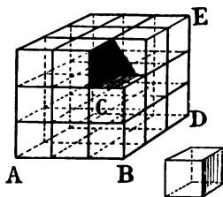
FIG. 6.—Showing a cubic yard and a cubic foot.
