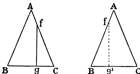
FIG. 23.—To show that the angles at the base of an isosceles triangle are equal.
