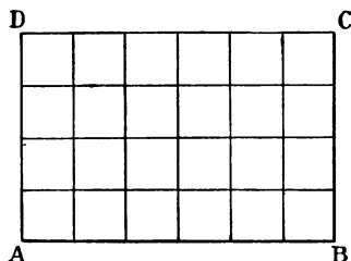
FIG. 31.—Product of two numbers.
