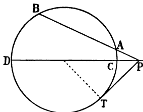
FIG. 28.— PB \times PA = PT^2 .
