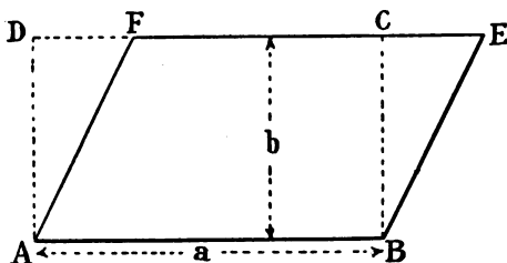
FIG. 114.—Area of a triangle.
