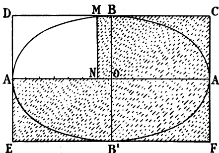
FIG. 131.—Area of an ellipse obtained experimentally.
